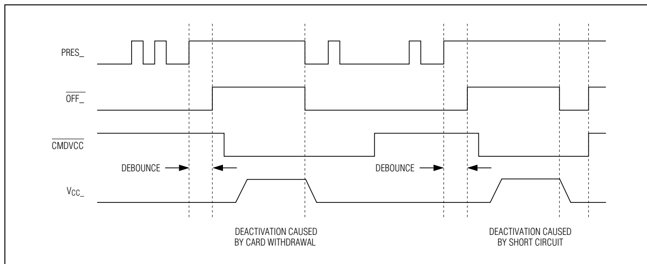
Figure 6. Behavior of PRES_, OFF_, CMDVCC, and VCC_
