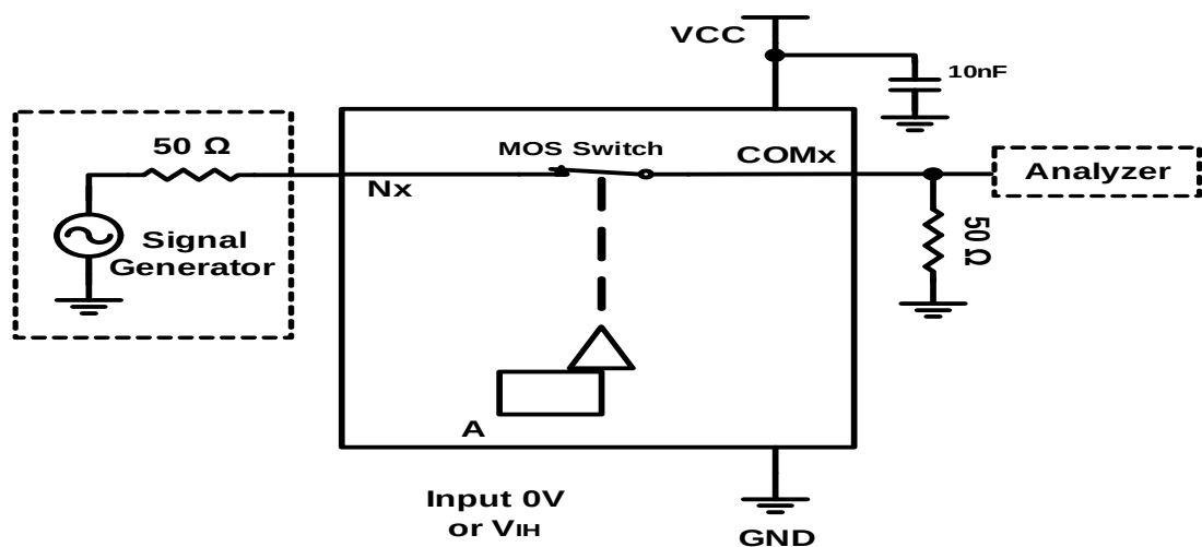
Figure8. -3dB Bandwidth ( f_{3dB} )
