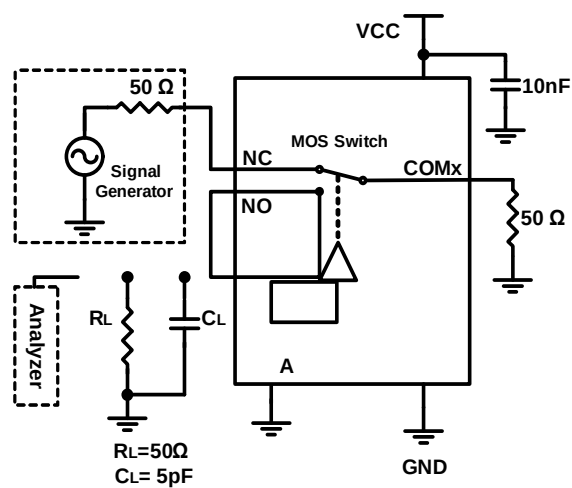
Figure5. Cross Talk ( V_{CT} )
