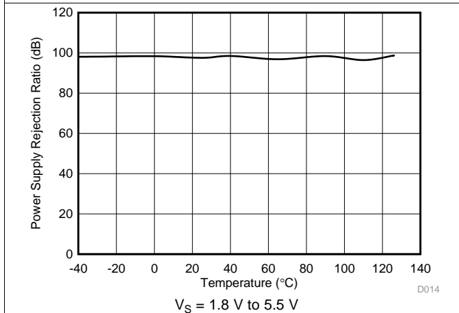
Figure 9. DC PSRR vs Temperature
