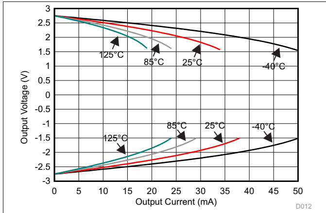
Figure 7. Output Voltage vs Output Current (Claw)
