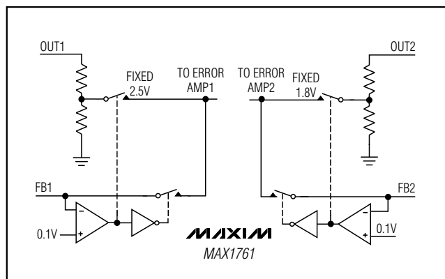
Figure 11. Feedback MUX
