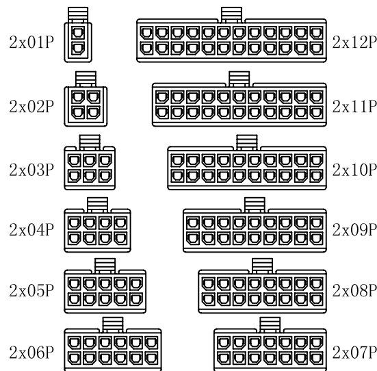
CIRCUIT SIZE LAYOUT
