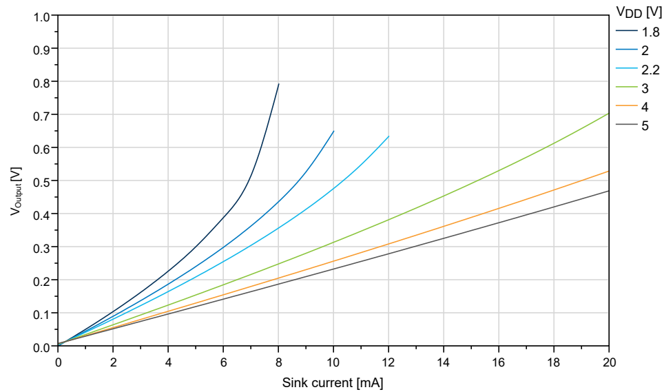
Figure 34-8. I/O Pin Output Voltage vs. Sink Current ( T = 25^{\circ}C )
