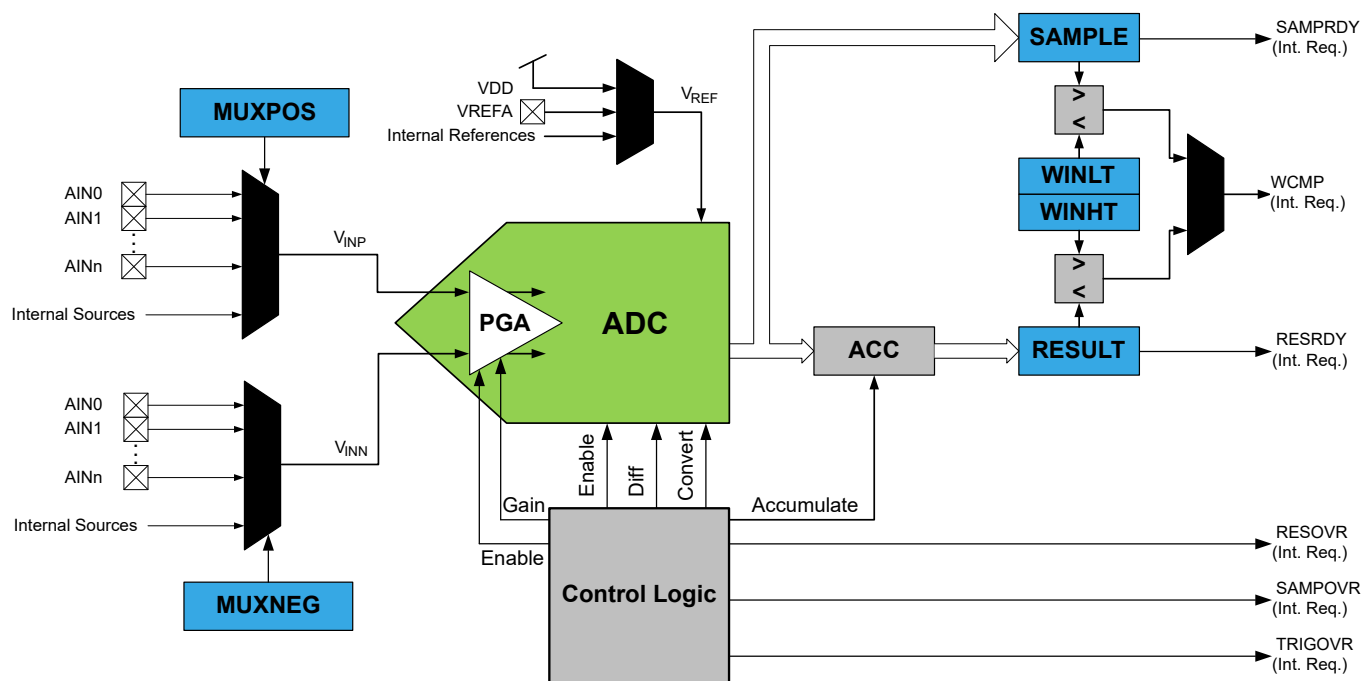
Figure 30-1. Block Diagram
