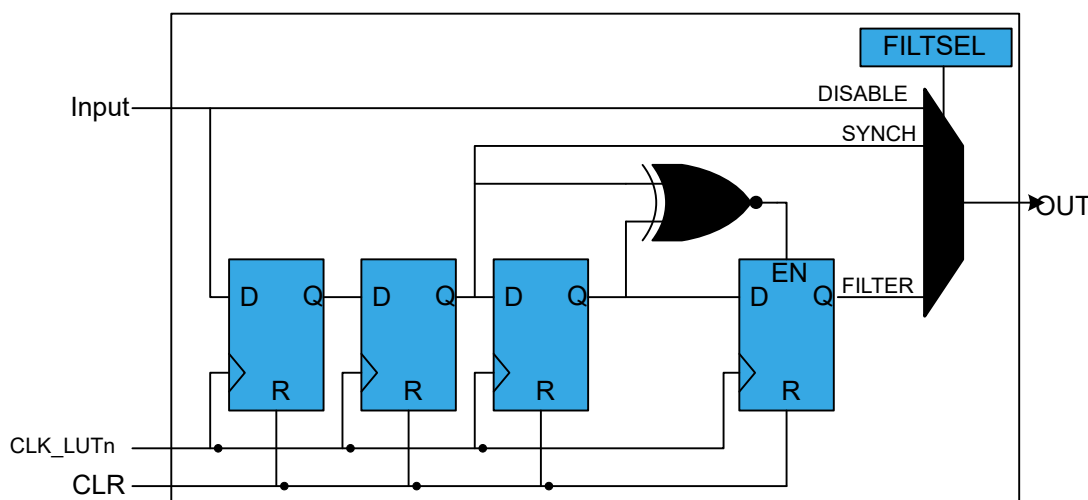
Figure 28-5. Filter
