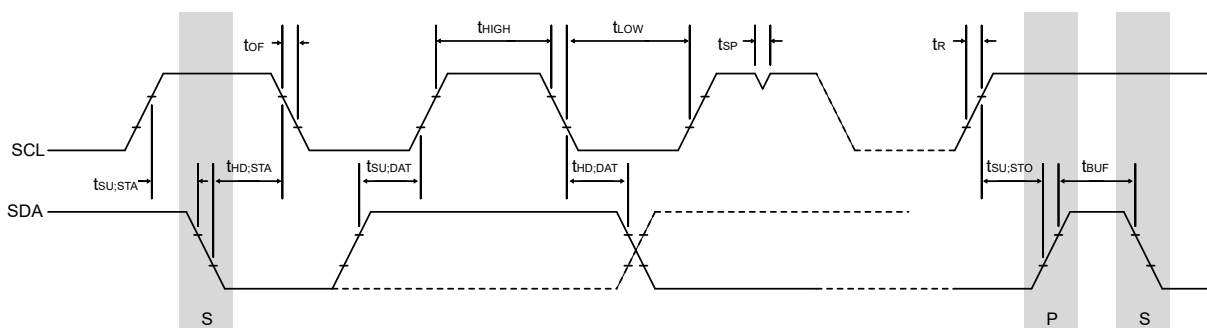
Figure 26-3. SCL Timing
