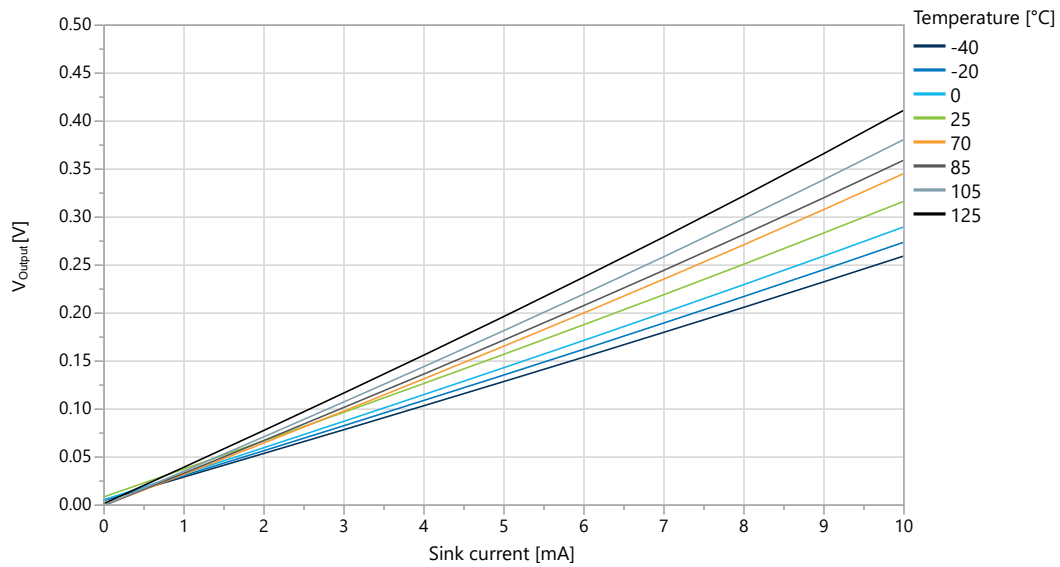
Figure 34-6. I/O Pin Output Voltage vs. Sink Current ( V_{DD} = 3.0V )
