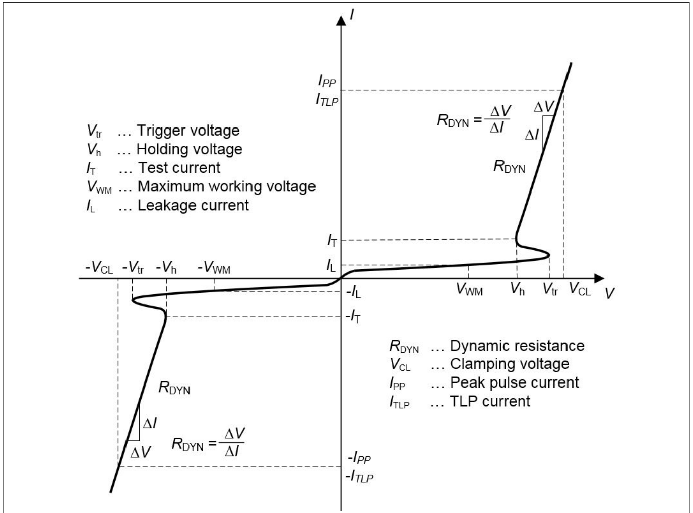
Figure 2 Definition of electrical characteristics
