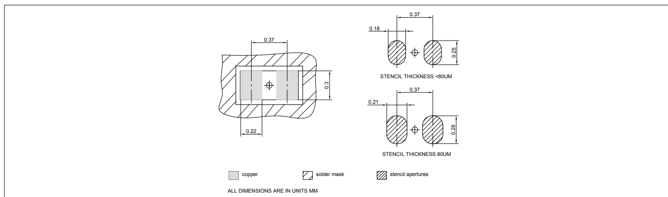
Figure 13 Footprint
