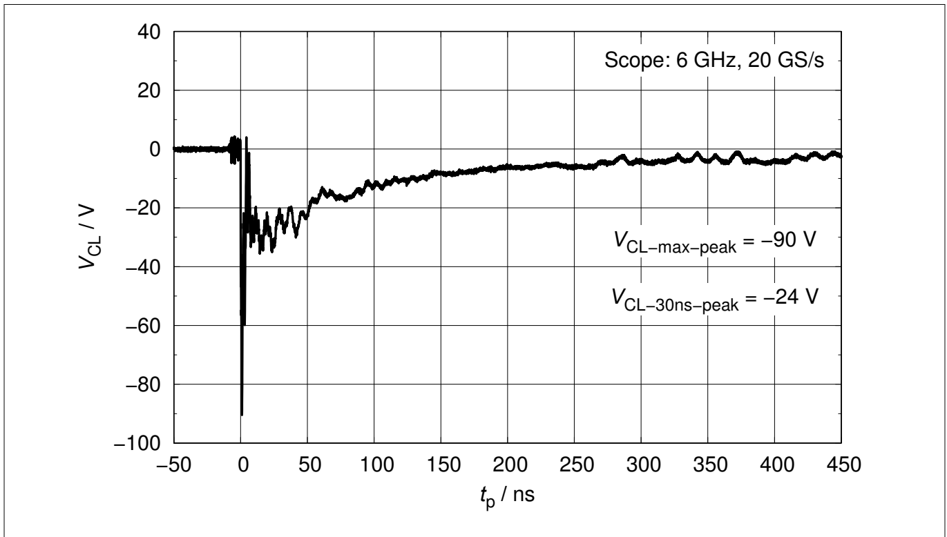
Figure 8 Clamping voltage (ESD): V_{CL} = f(t) , 15 kV negative pulse 7)
