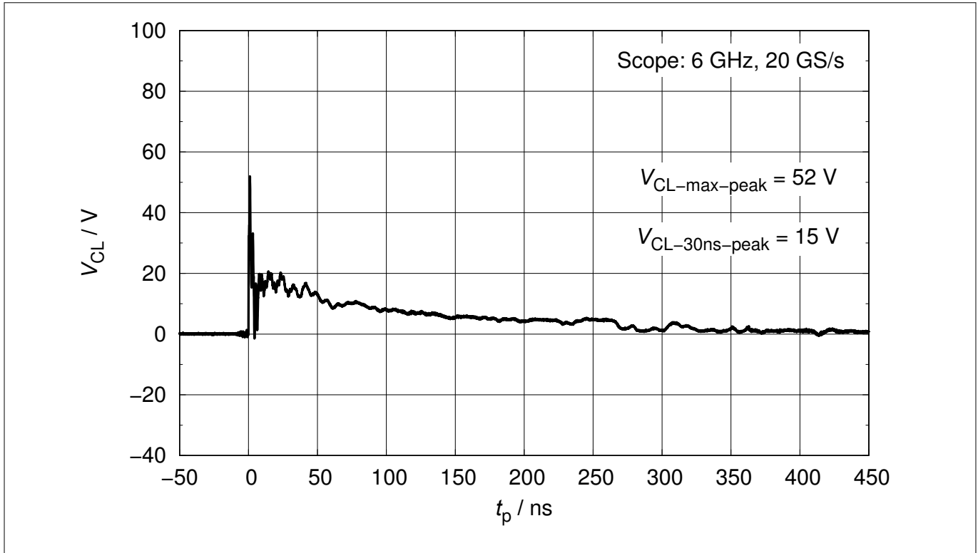
Figure 5 Clamping voltage (ESD): V_{CL} = f(t) , 8 kV positive pulse 7)
