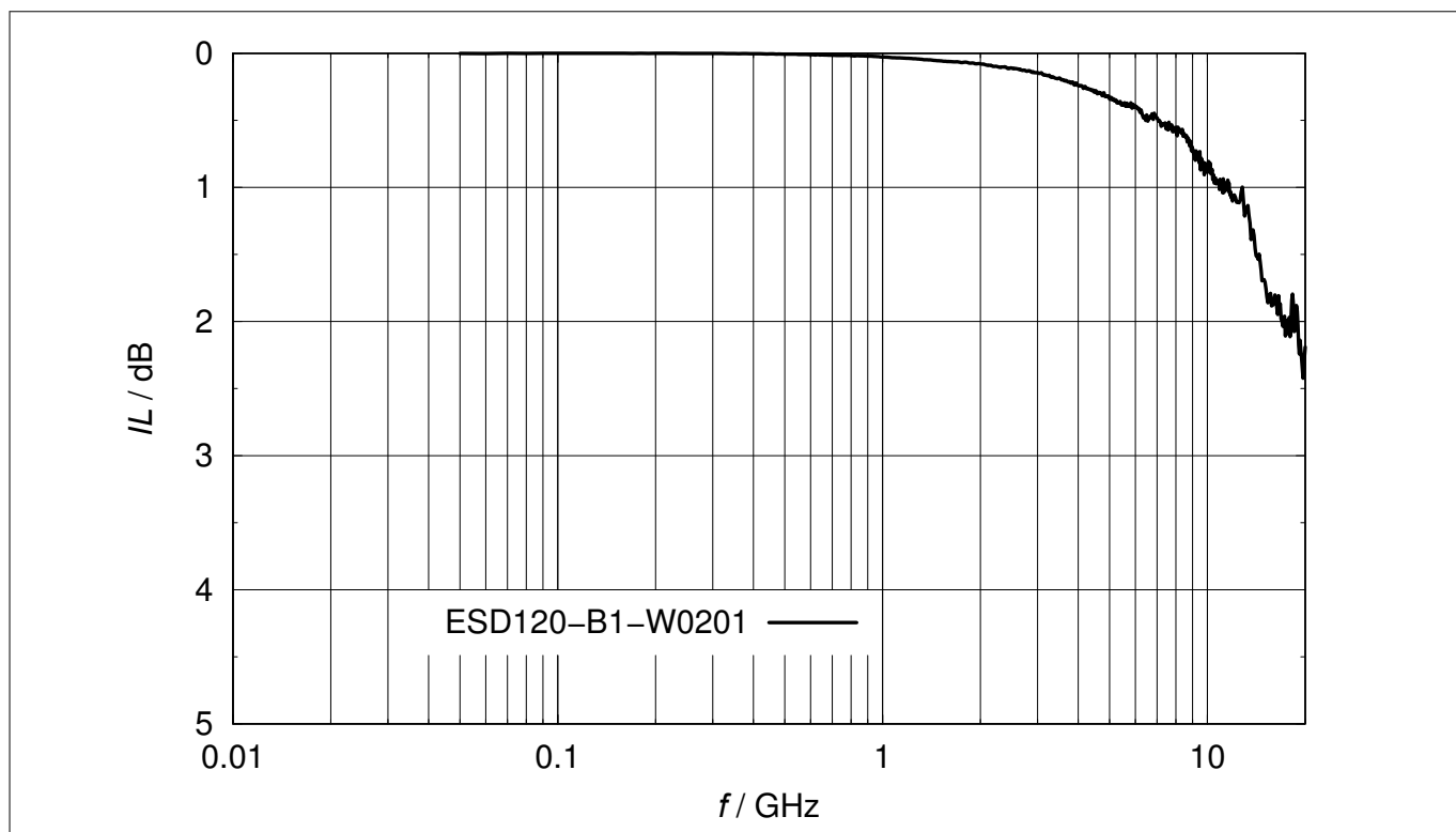
Figure 11 Insertion loss IL = f(f)
