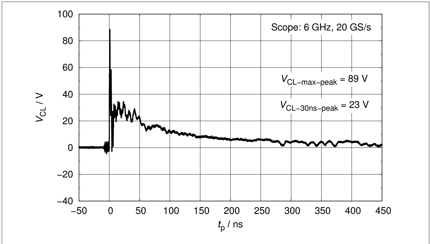
Figure 7 Clamping voltage (ESD): V_{CL} = f(t) , 15 kV positive pulse 7)
