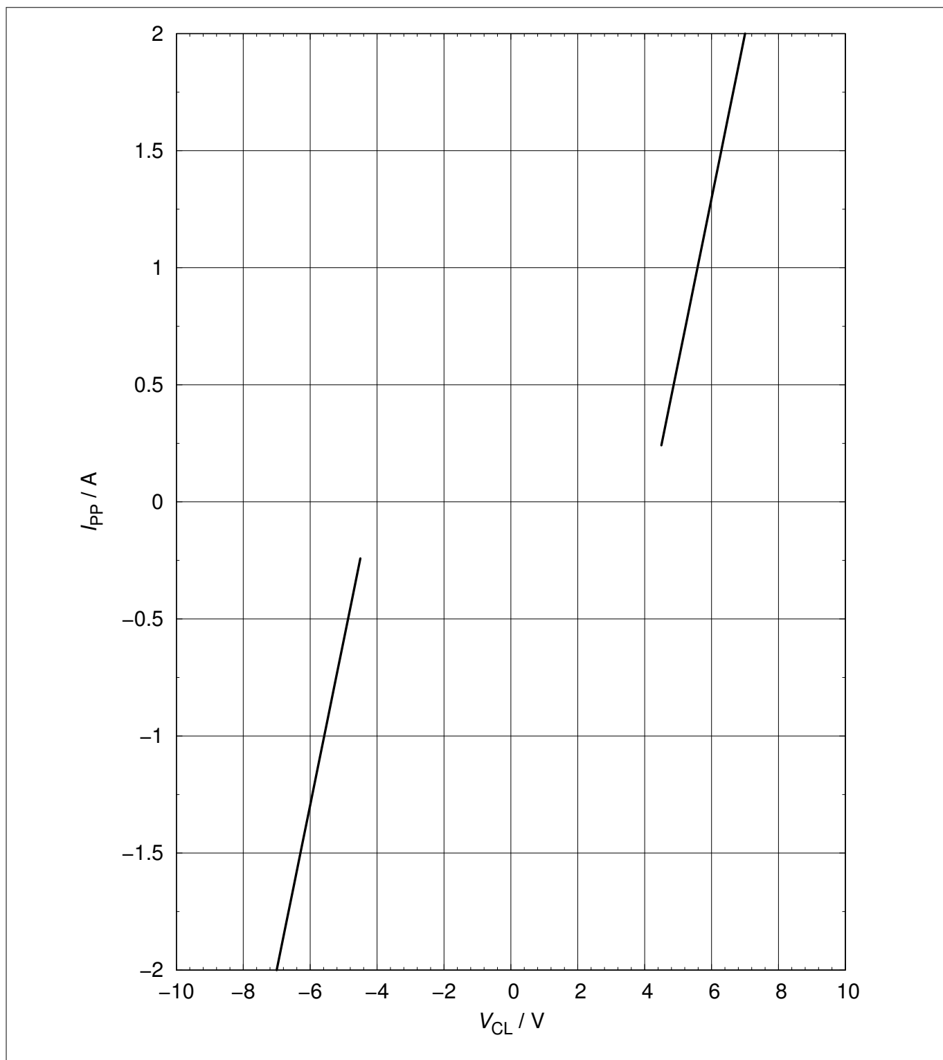
Figure 10 Clamping voltage (Surge): I_{PP} = f(V_{CL}) 8) [1]
