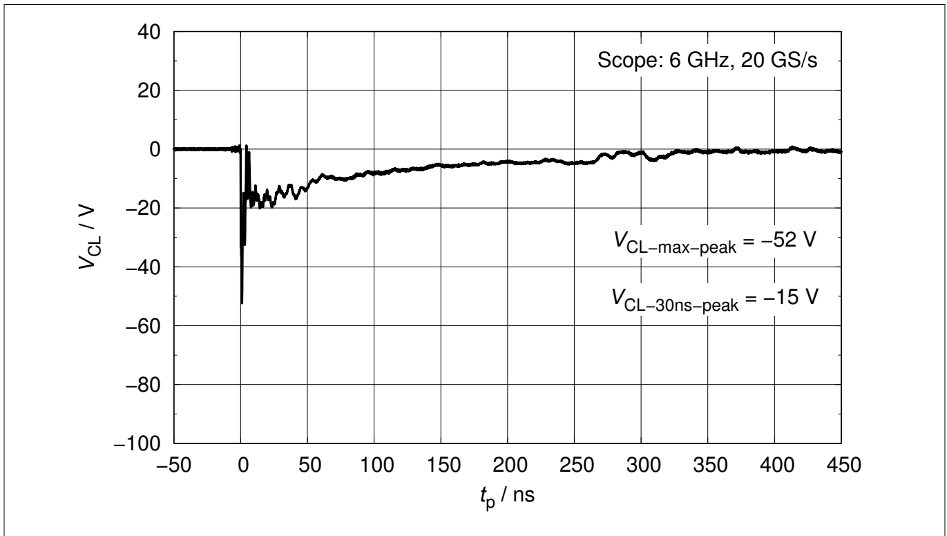
Figure 6 Clamping voltage (ESD): V_{CL} = f(t) , 8 kV negative pulse 7)
