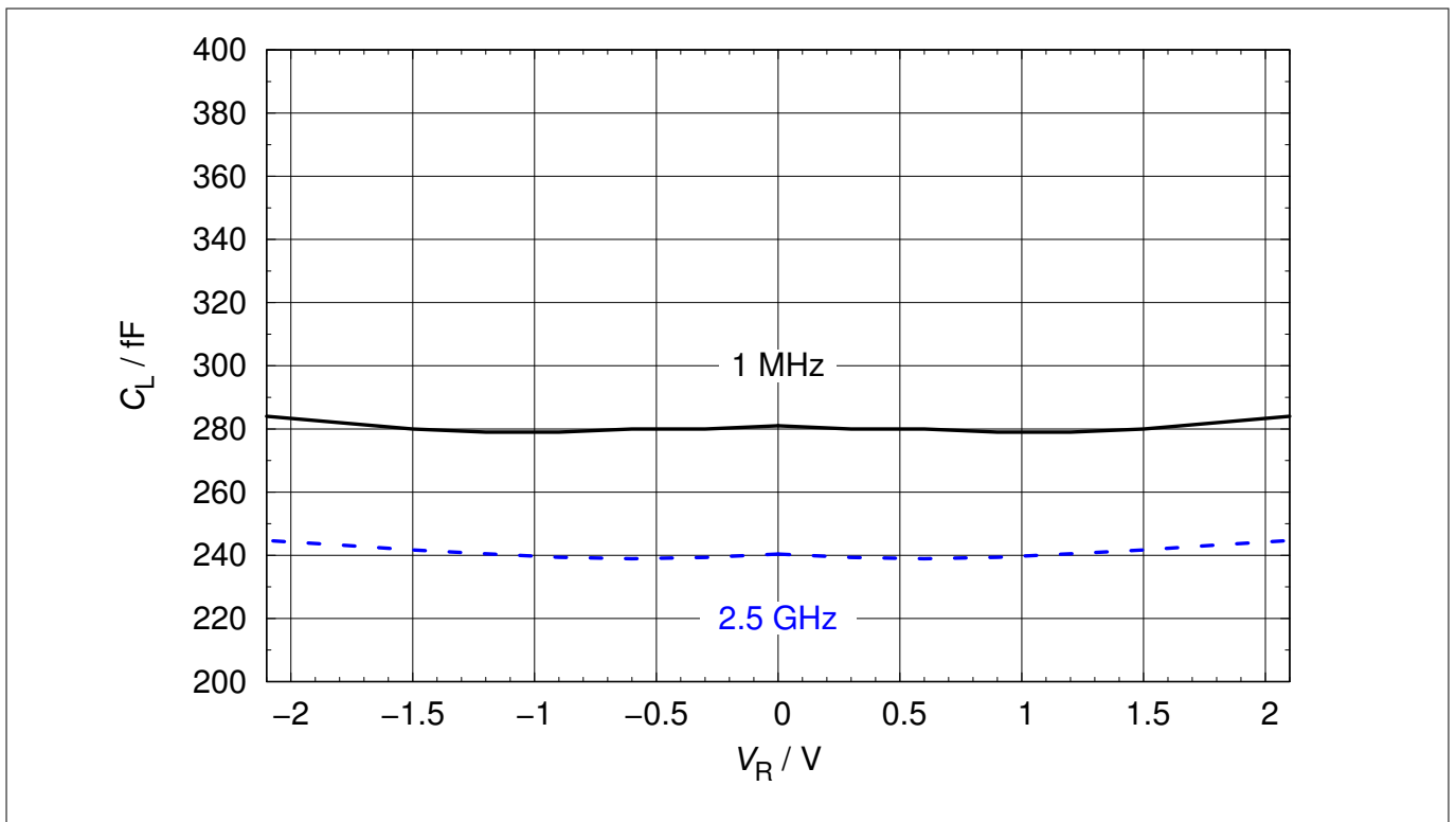
Figure 4 Line capacitance: C_L = f(V, f = 1\text{ MHz}, 2.5\text{ GHz})
