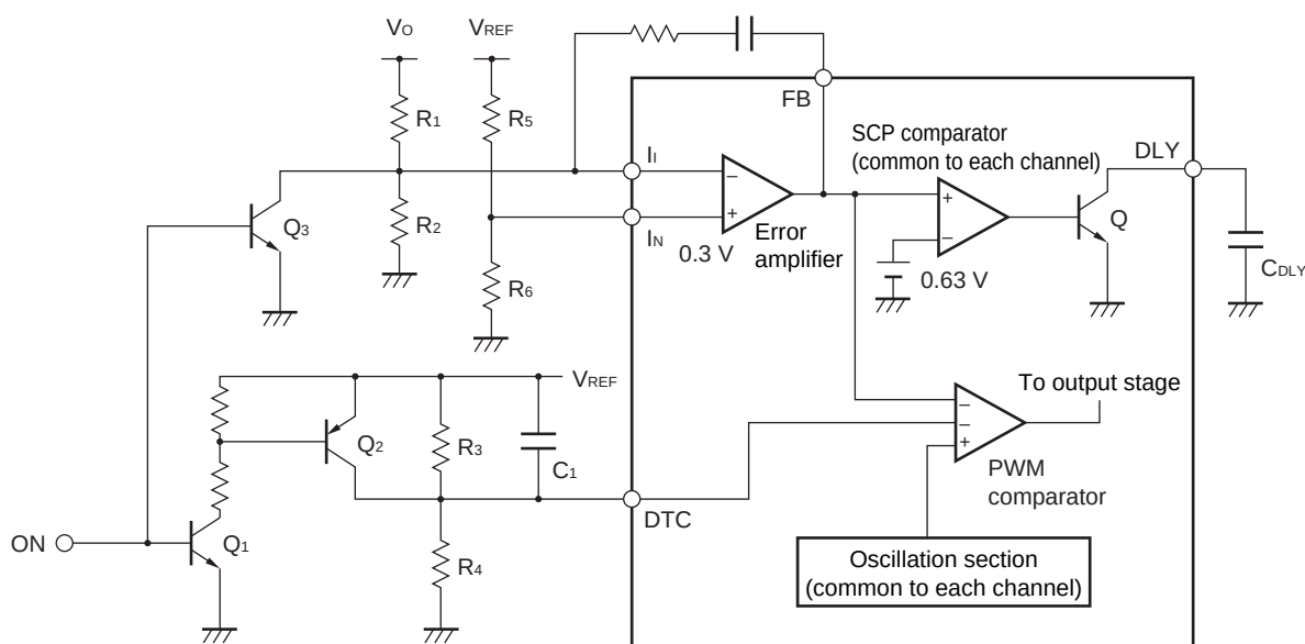
Figure 3-3 ON/OFF Control
