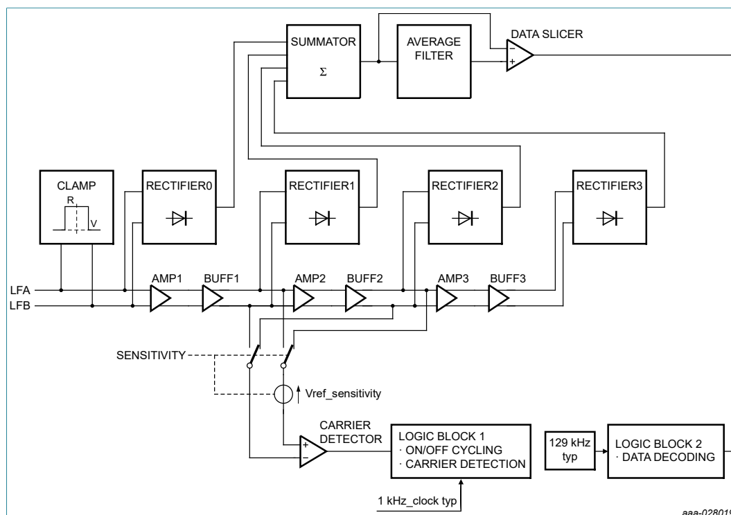
Figure 26. Block diagram
