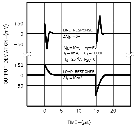
FIGURE 6. TRANSIENT RESPONSE
