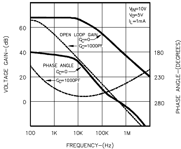
FIGURE 5. FREQUENCY RESPONSE
