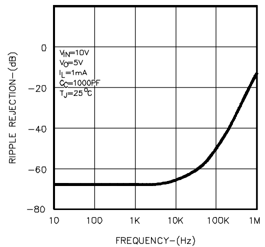
FIGURE 4. RIPPLE REJECTION
