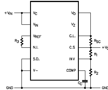
FIGURE 10 - BASIC LOW CURRENT REGULATOR
