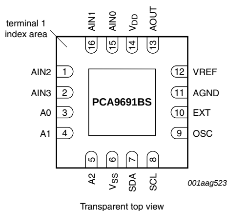
Fig 2. Pin configuration for HVQFN16 (PCA9691BS)
