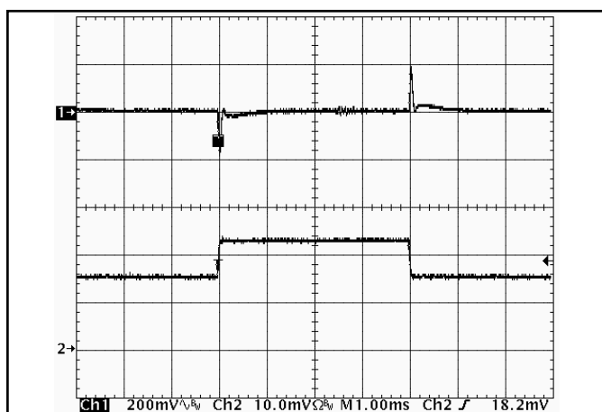
Figure 15: Output voltage response to step-change in load current (50%-75%-50% of Iout(max); dI/dt = 0.1A/\mu s ). Load cap: 10 \mu F, 100 m \Omega ESR tantalum cap and 1 \mu F ceramic cap. Ch 1: Vout (200mV/div), Ch 2: Iout (10A/div).
