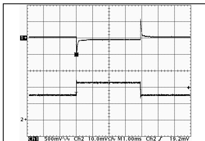
Figure 16: Output voltage response to step-change in load current (50%-75%-50% of Iout(max); dI/dt = 5A/\mu s ). Load cap: 470 \mu F, 30 m \Omega ESR tantalum cap and 1 \mu F ceramic cap. Ch 1: Vout (500mV/div), Ch 2: Iout (10A/div).
