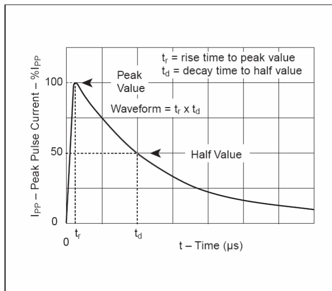
Figure2 t_r \times t_d Pulse Wave-form
