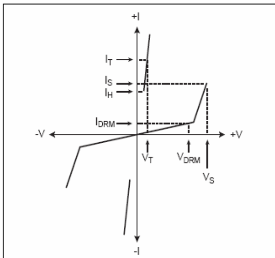
Figure1 V-I Characteristics
