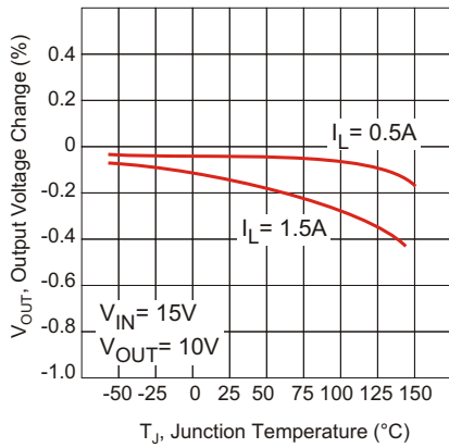
Figure 1. Load Regulation
