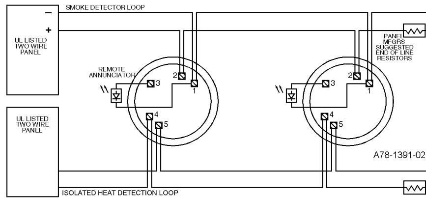
Figure 4. Wiring diagram for 2400AIT detector with isolated thermal and two-wire panels:
