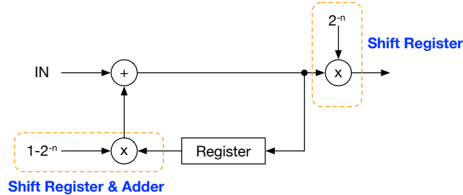
图 7. Single Pole Digital Filter Implementation
