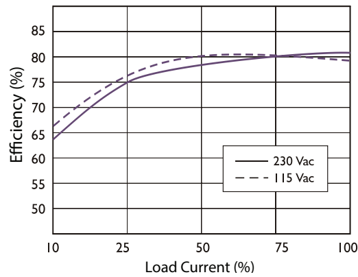
PDR-10-24 Efficiency Curve (Efficiency vs. Load Current)
