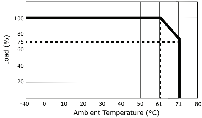
Temperature Derating Curve (Output Load vs. Ambient Temperature)
