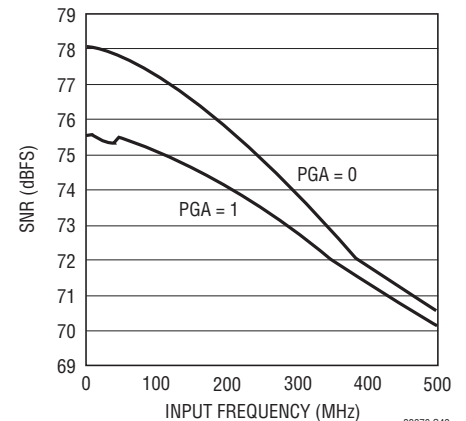
LTC2206: SNR vs Input Frequency, 80\text{Mpsps}
