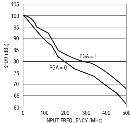
LTC2206: SFDR (HD2 and HD3) vs Input Frequency, 80\text{Mpsps}
