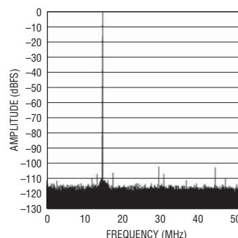
LTC2207: 64K Point FFT, f IN = 14.8MHz, -1dBFS, PGA = 0, 105Msps
