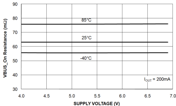
Figure 14. V_{BUS} On Resistance ( m\Omega ) vs. Supply Voltage
