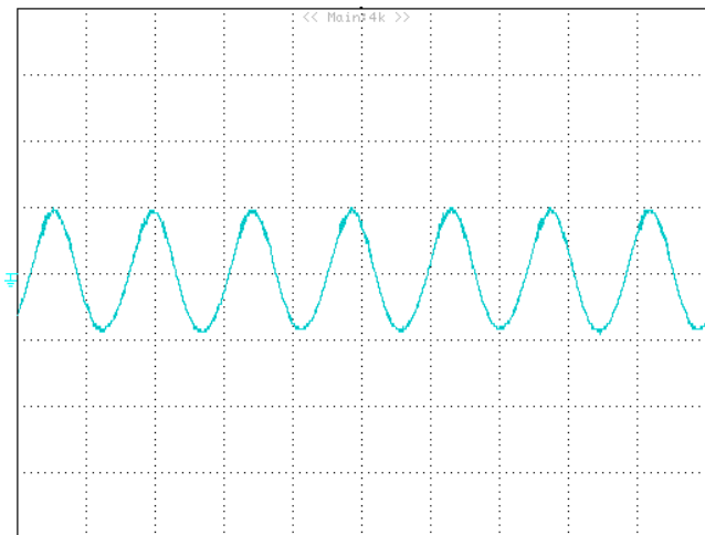
Figure 14: Output voltage ripple at nominal input voltage and rated load current ( I_o=25\text{A} ) ( 50\text{mV}/\text{div} , 2\mu\text{s}/\text{div} ) Load capacitance: 220\mu\text{F} (Electrolytic) + 10\mu\text{F} (Tantalum) + 1\mu\text{F} (Ceramic) and min Co. Bandwidth: 20\text{MHz} .
