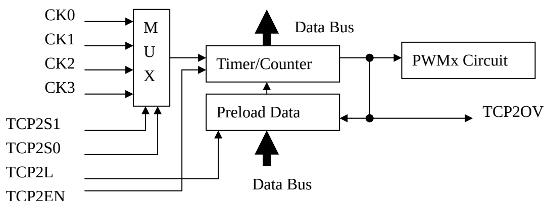
Figure: Timer/Counter/PWM
