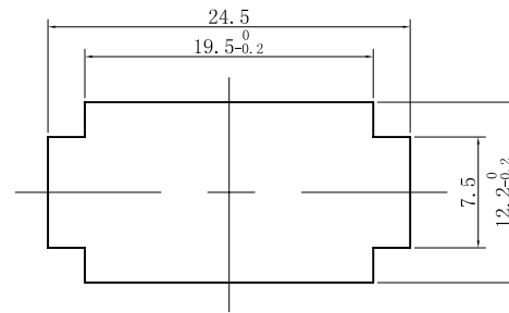
PANEL CUT-OUT
