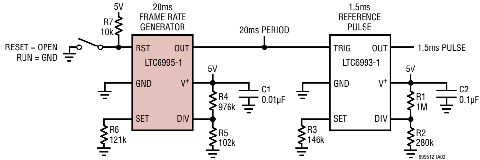
1.5ms Radio Control Servo Reference Pulse Generator
