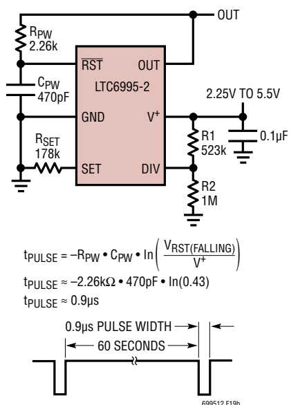
Figure 19b. Self-Resetting Circuit (DIVCODE = 11)
