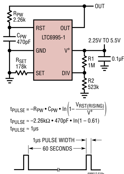
Figure 19a. Self-Resetting Circuit (DIVCODE = 4)
