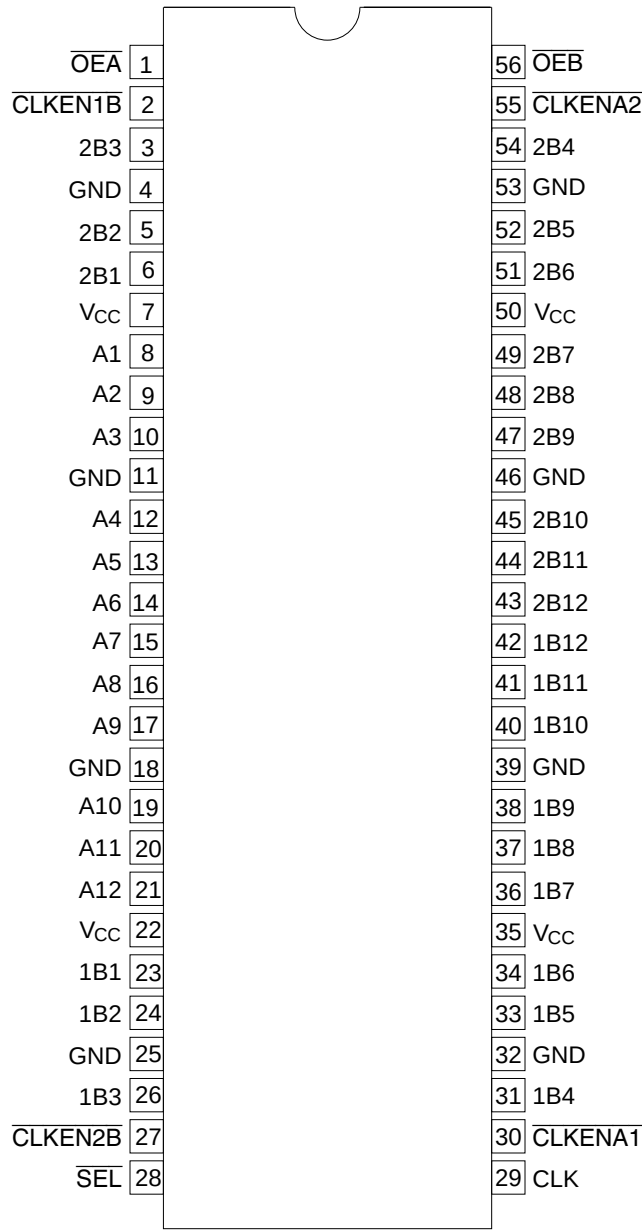
(Top view)
