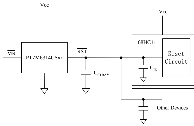
Fig 6. PT7M6314USxx Application Example
