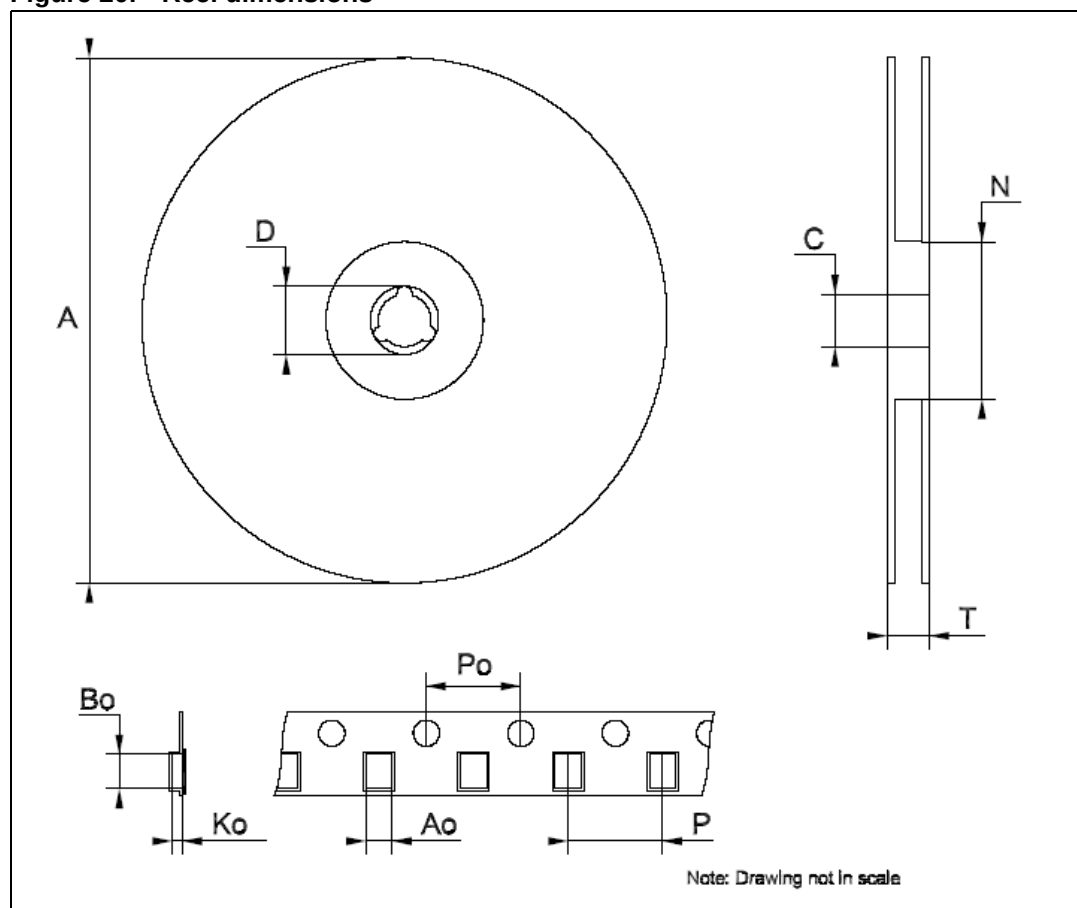
Figure 20. Reel dimensions
