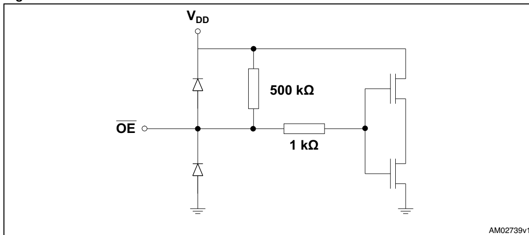
Figure 5. \overline{OE} terminal
