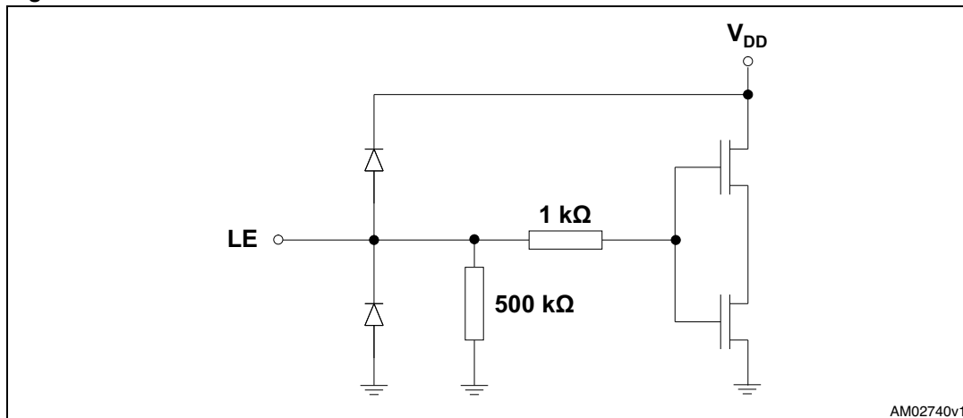
Figure 6. LE terminal
