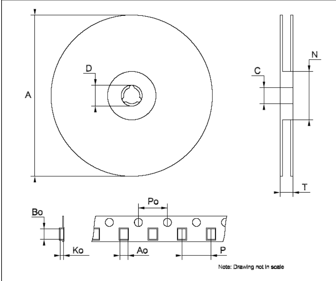
Figure 22. Reel dimensions
