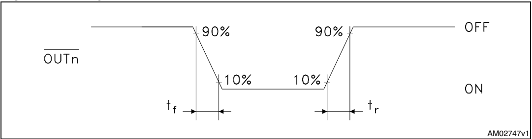
Figure 14. Outputs
