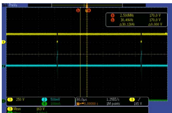
Short circuit protection test
