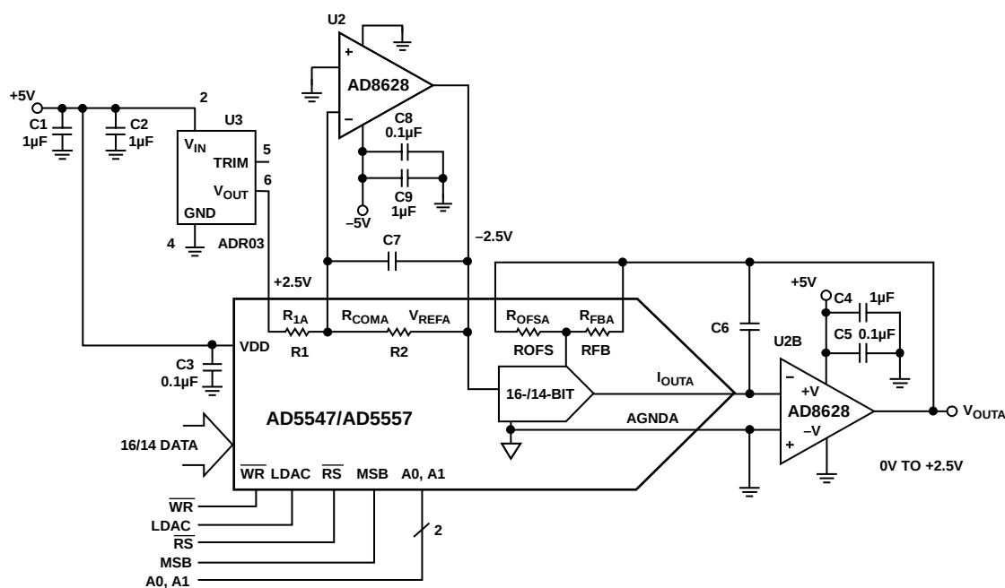
Figure 22. Unipolar 2-Quadrant Multiplying Mode, V_{OUT} = 0 to +V_{REF}
