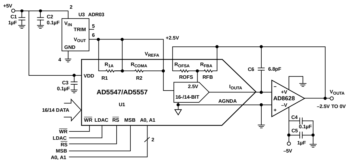
Figure 21. Unipolar 2-Quadrant Multiplying Mode, V_{OUT} = 0 to -V_{REF}
