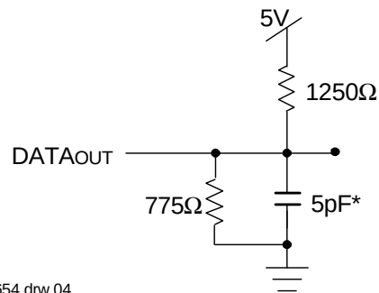
Figure 2. Output Test Load (For t IZ , t HZ , t WZ , t OW ) *Including scope and jig.
