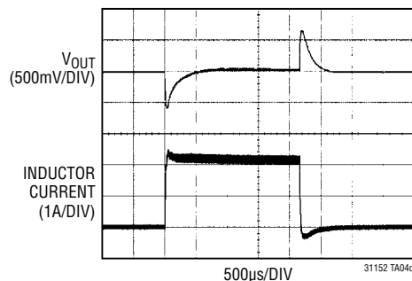
0A to 1.5A Load Step, V_{IN} = 10.6V
