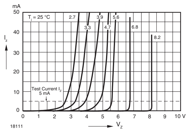
Figure 12. Breakdown Characteristics
