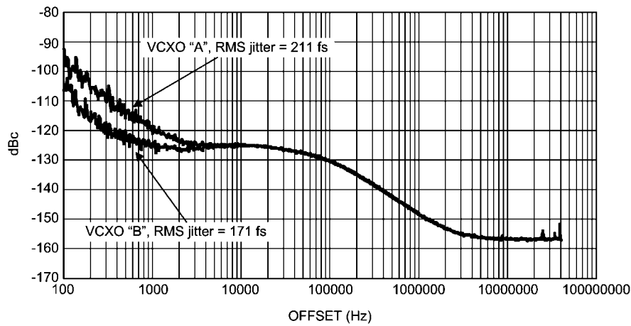
FIGURE 24. LVPECL Clock Output Phase Noise Comparison, 250 MHz
