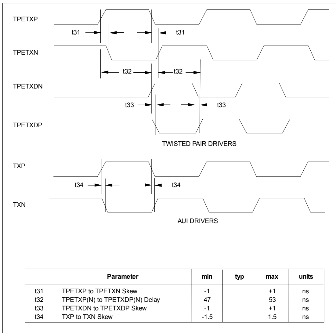
Figure 12.10 – Differential Output Signal Timing (10BASE-T and AUJ)
