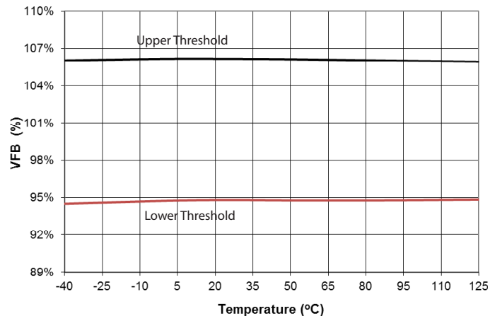
PG Threshold
