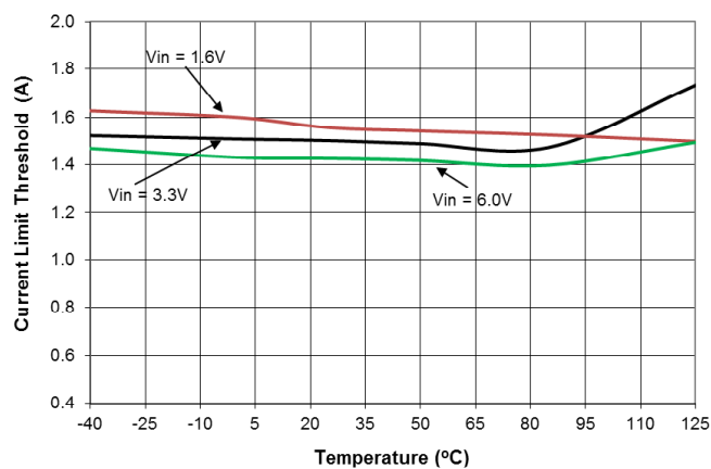
Current Limit Threshold
