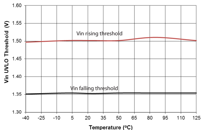
Input Under-voltage Lockout Threshold
