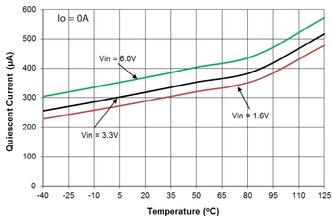
Quiescent Current
