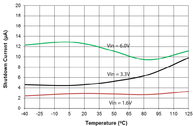
Shutdown Current
