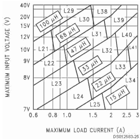
FIGURE 5. LM2596-5.0
