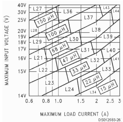
FIGURE 6. LM2596-12
