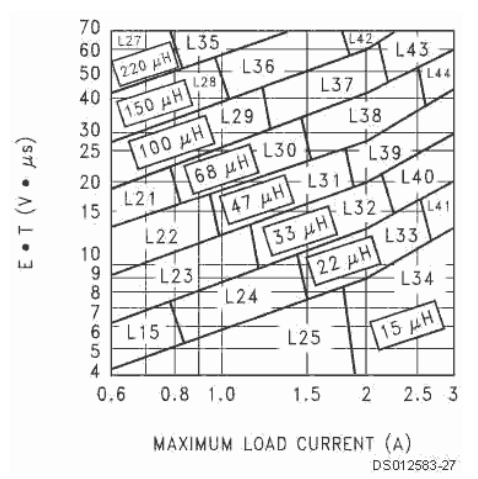
FIGURE 7. LM2596-ADJ
