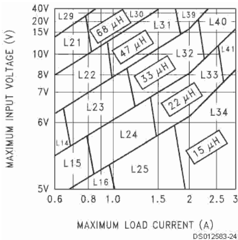
FIGURE 4. LM2596-3.3
