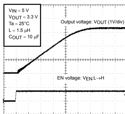
Startup Characteristics ( C_{SS} = 0.1\text{ }\mu\text{F} )
