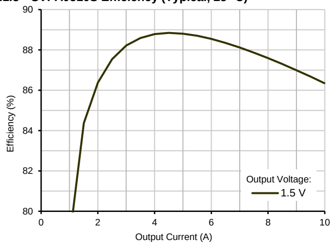
4.1.3 SVFA0510S Efficiency (Typical, 25 °C)
