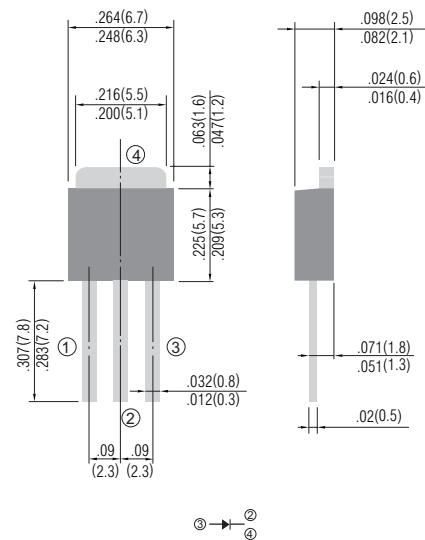
TO-251AB
