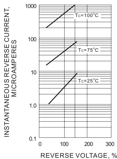
Fig.3-TYPICAL REVERSE CHARACTERISTICS
