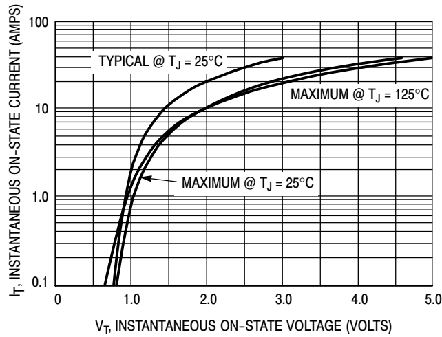
Figure 3. On-State Characteristics
