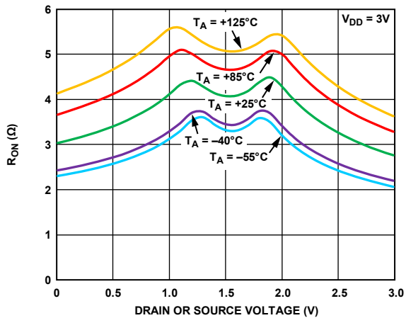
Figure 4. On Resistance vs. V_D ( V_S ) for Different Temperatures, V_{DD} = 3 V
