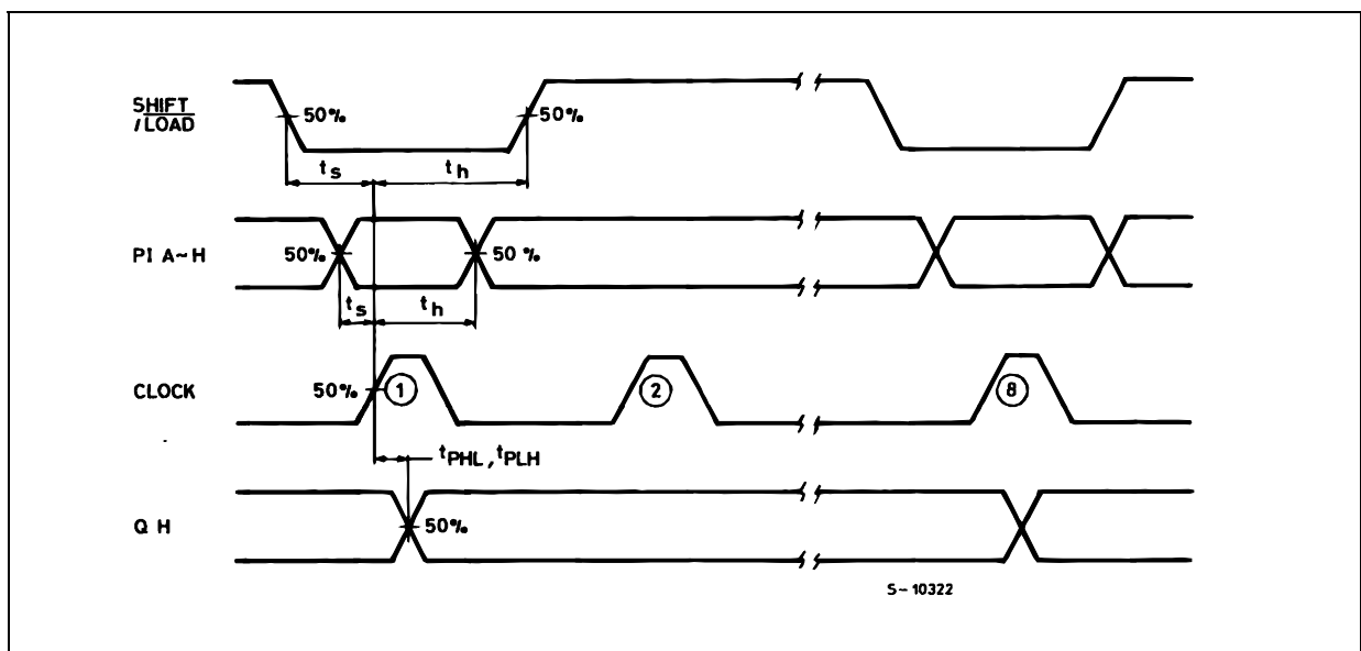
WAVEFORM 3: PROPAGATION DELAY TIME, SETUP AND HOLD TIME (PI, \overline{S/L} to CLOCK) ( f=1\text{MHz} ; 50% duty cycle)
