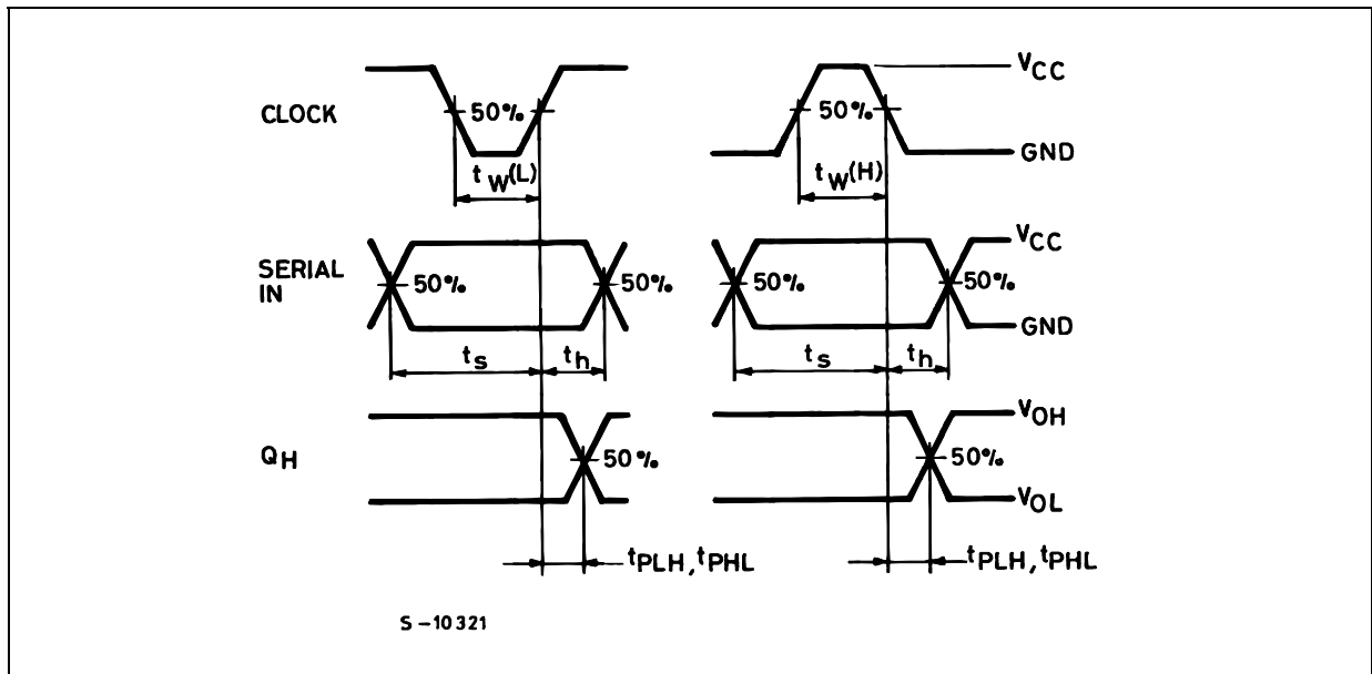
WAVEFORM 2: PROPAGATION DELAY TIME, MINIMUM PULSE WIDTH (CLOCK), SETUP AND HOLD TIME (SI to CLOCK) ( f=1\text{MHz} ; 50% duty cycle)
