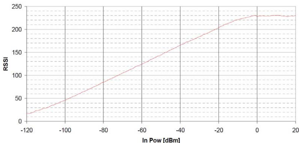
Figure 3: RSSI vs Input Power
