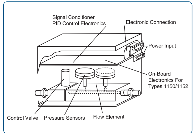
Figure 2 — Component Assembly
