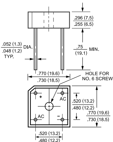
KBPC-8/10
