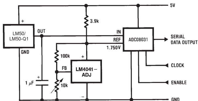
Figure 19. Temperature To Digital Converter (Serial Output) (+125 ^{\circ}\text{C} Full Scale)
