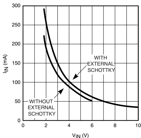
Figure 6. No Load Input Current vs. Input Voltage for the Circuit of Figure 7
