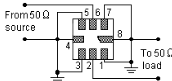
Test Circuit
