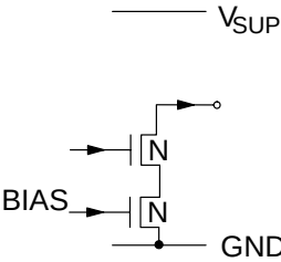
Fig. 4-14: Output pins 40, 42, 44
