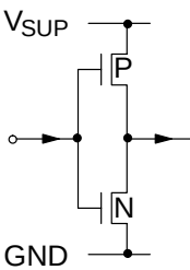
Fig. 4-5: Input pins 2, 3
