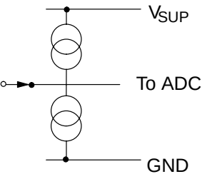
Fig. 4-16: Input pin 59, 61, 63
