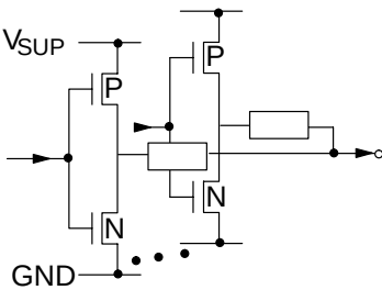
Fig. 4-11: Output pins 33, 35
