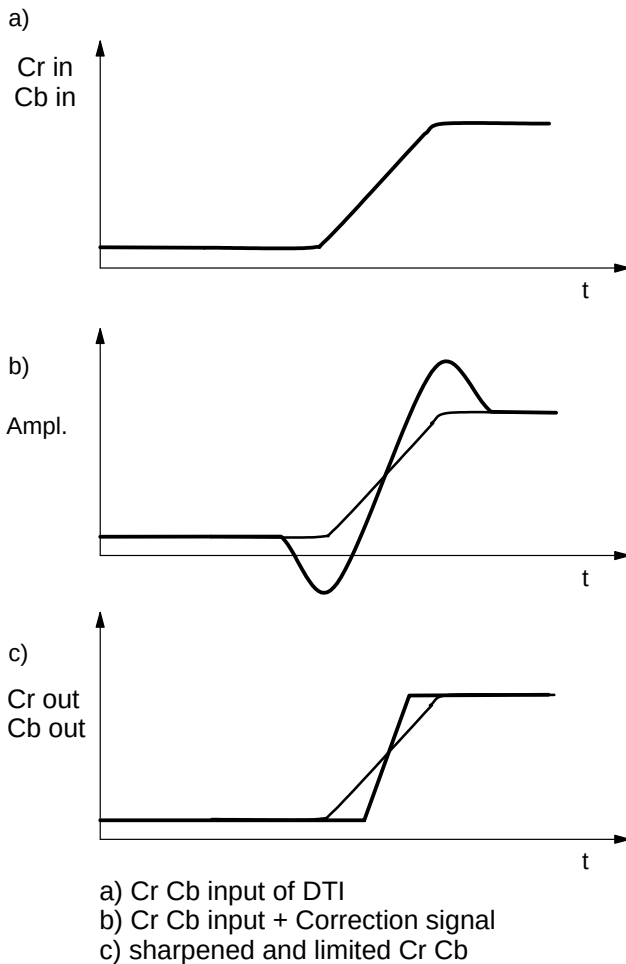
Fig. 2-21: Digital Color Transient Improvement
