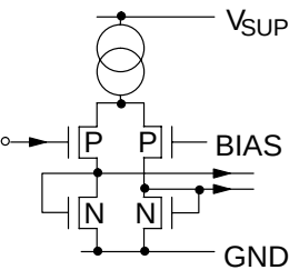
Fig. 4-12: Input pins 34, 36, 38, 65, 66, 67
