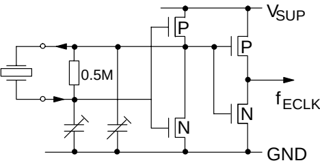
Fig. 4-10: Input pins 17, 18
