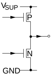
Fig. 4-6: Output pin 4, 10
