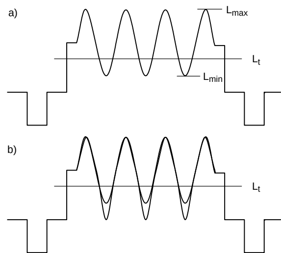
Fig. 2–15: Black-level-expansion
