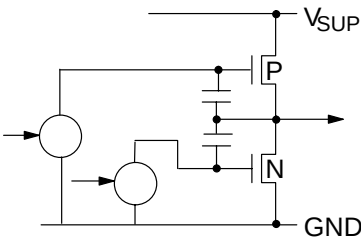
Fig. 4-7: Output pin 55
