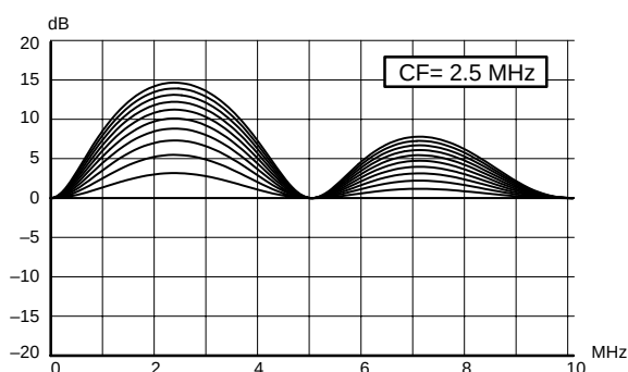
Fig. 2–16: Dynamic peaking frequency response
