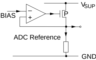
Fig. 4-17: Pin 62
