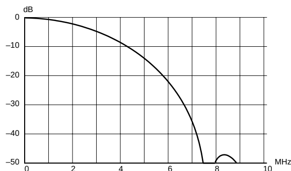
Fig. 2-20: Frequency response of the chroma interpolation filter
