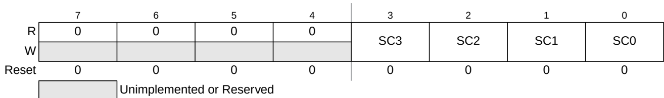
Figure 19-10. Debug State Control Register 1 (DBGSCR1)
