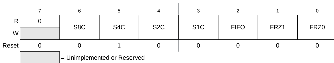
Figure 4-6. ATD Control Register 3 (ATDCTL3)
