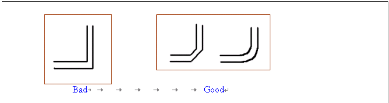
Figure 10 Trace routing
